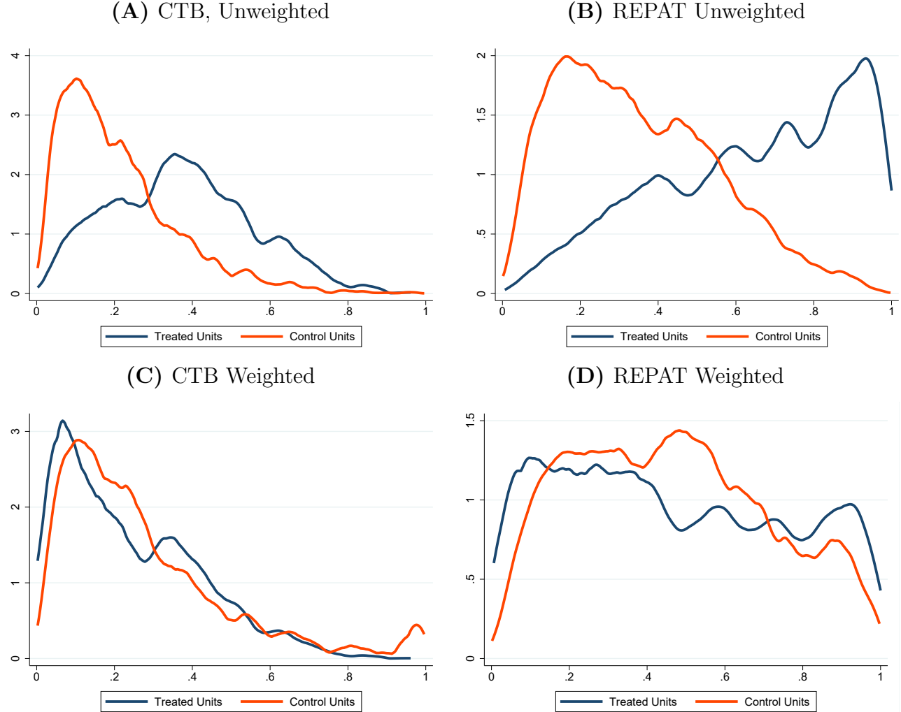
Figure E1: Assessing Matching Strategies using Kernel Density Plots
